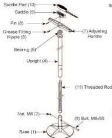
Figure 1 - Model MPS1500A Components
